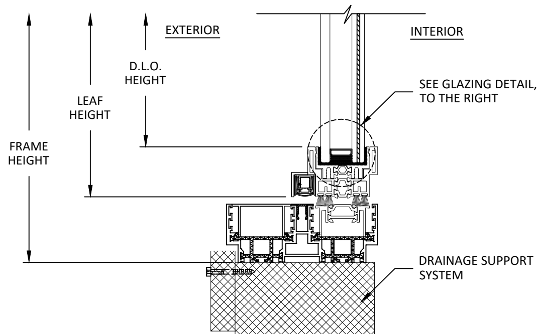
B 4 VERTICAL SECTION SILL
