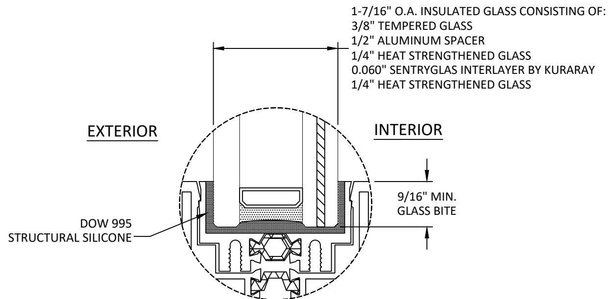
GLAZING DETAIL 1
